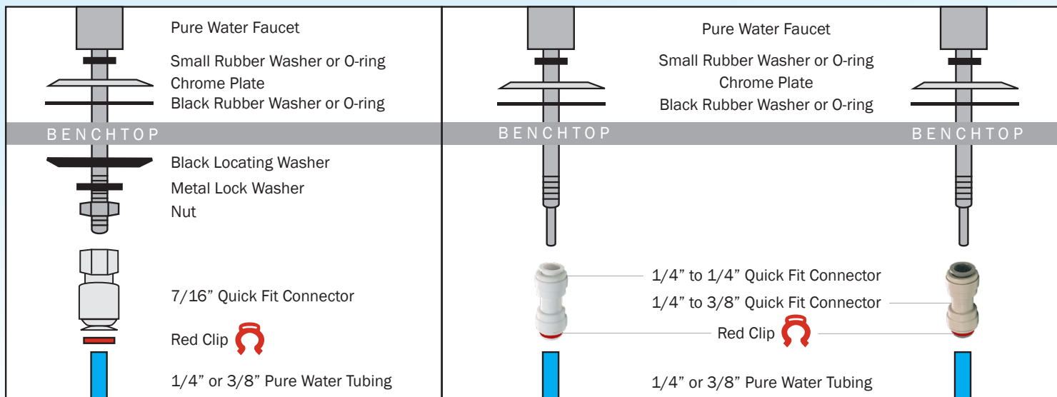
Diagram 4 - Faucet Installation
