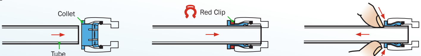
Diagram 3 - Tube Connections
