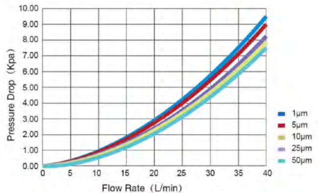
DLS Filter Pressure Drop vs. Flow Rate @ 20°C
